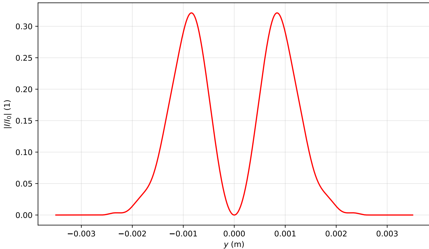
Intensity profile I(x=0, y, z=3.184)/I_0 , P_{in}=2.0P_{cr} , artificial time
